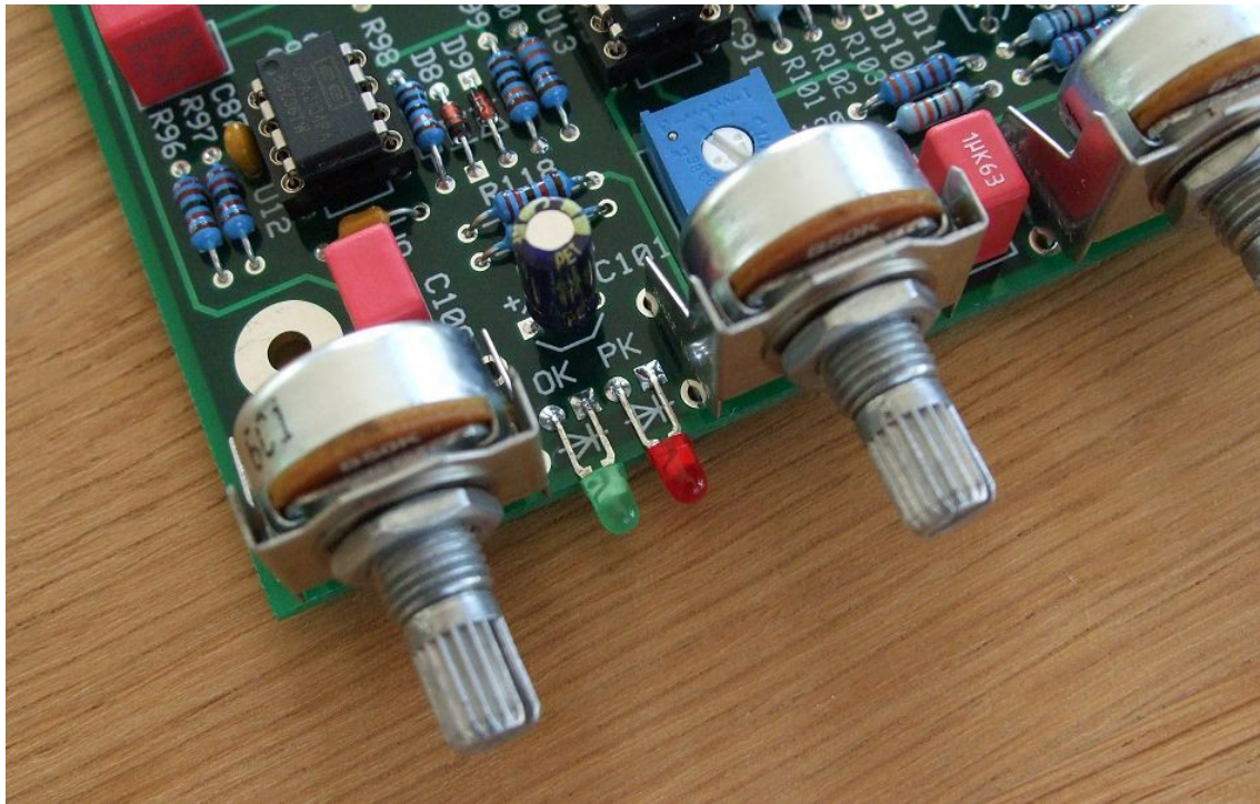
The signal OK and Peak LEDs. The cathode is denoted by the square pad on the PCB and the larger triangular section within the LED's translucent plastic body.
