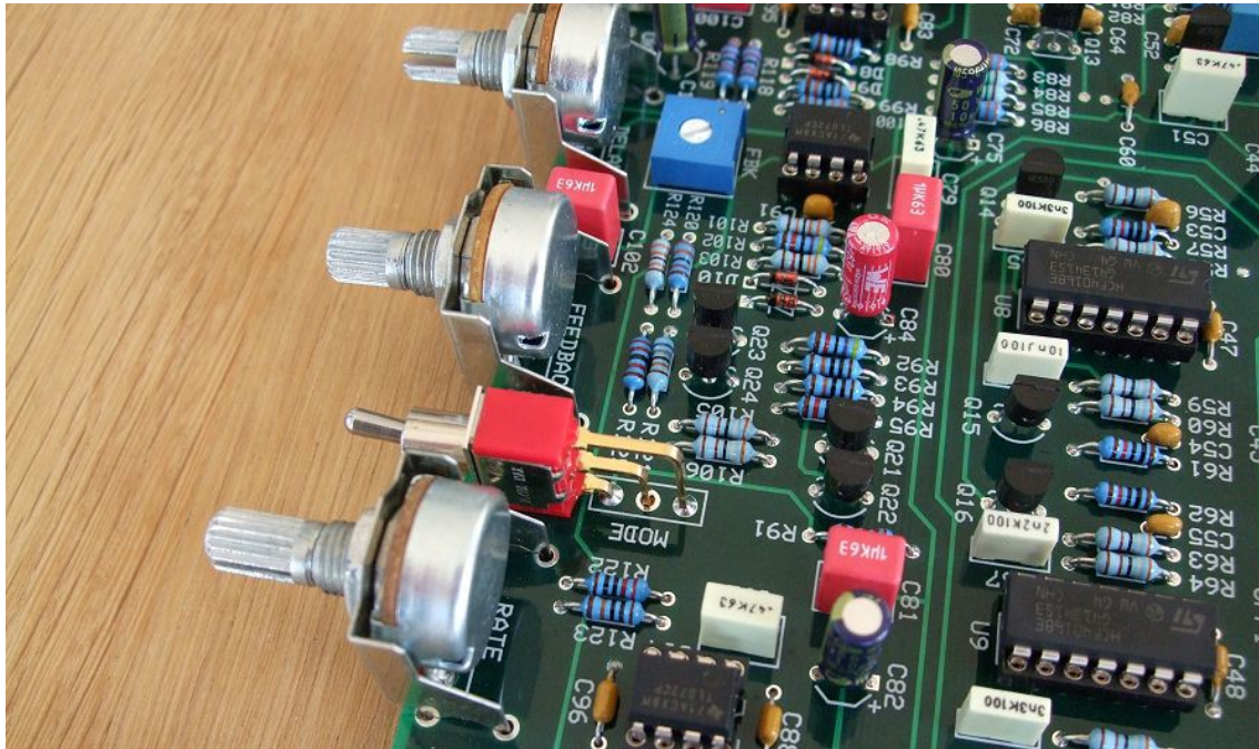
The switch here is Multicomp's two position 1MS1T2B4M7RE
