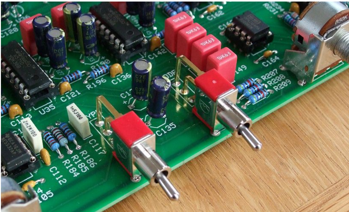
These switches are Multicomp's ON-ON 1MS1T2B4M7RE, here shown on an SRE330 but the fitting on the DCR320 is similar.
